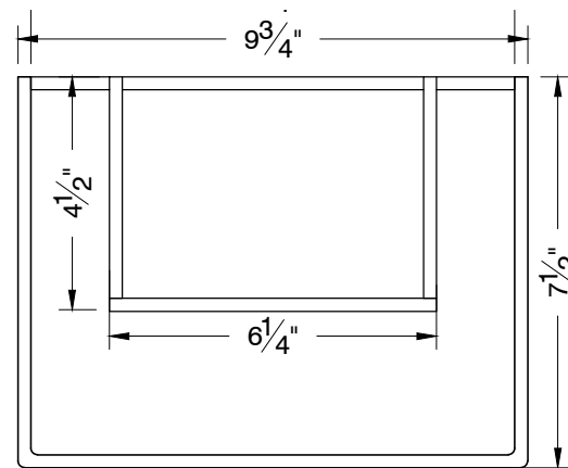
3 SECTION PART BOX & INNER TRAY SCALE 1:4
