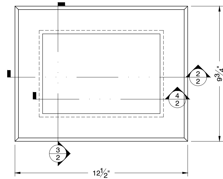
5 PLAN PART BOX & INNER TRAY SCALE 1:4
